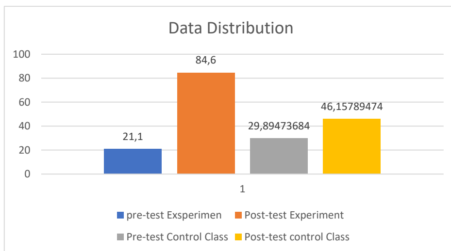
Figure 1 <Data Distribution>
